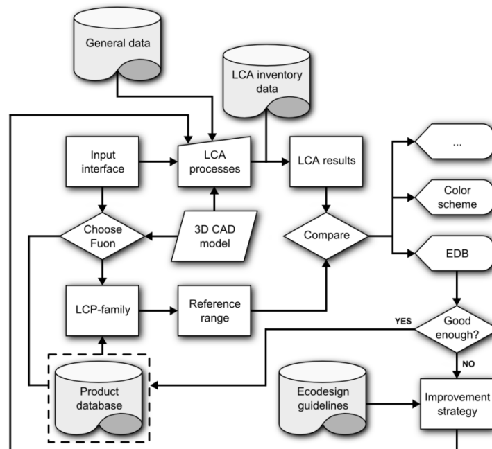
Figure 3: Database structure for CAD implementation (Ostad-Ahmad-Ghorabi, 2010)
